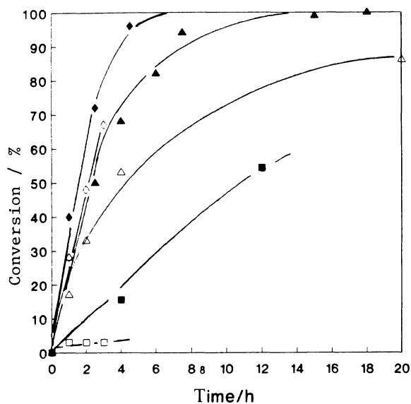
Fig. 1. Activity of [\text{Hf}]_5\text{-H} (filled symbols) and [\text{Zr}]_5\text{-H} (open symbols) for hydrogenolysis of neopentane. % wt: 3.1 (M=Hf); 1.5 (M=Zr); M/ \text{H}_2 / NpH: 1/ 300/ 60 (molar ratio); \square, \blacksquare at 323 K; \Delta, \blacktriangle at 373 K; \diamond, \blacklozenge at 423 K
